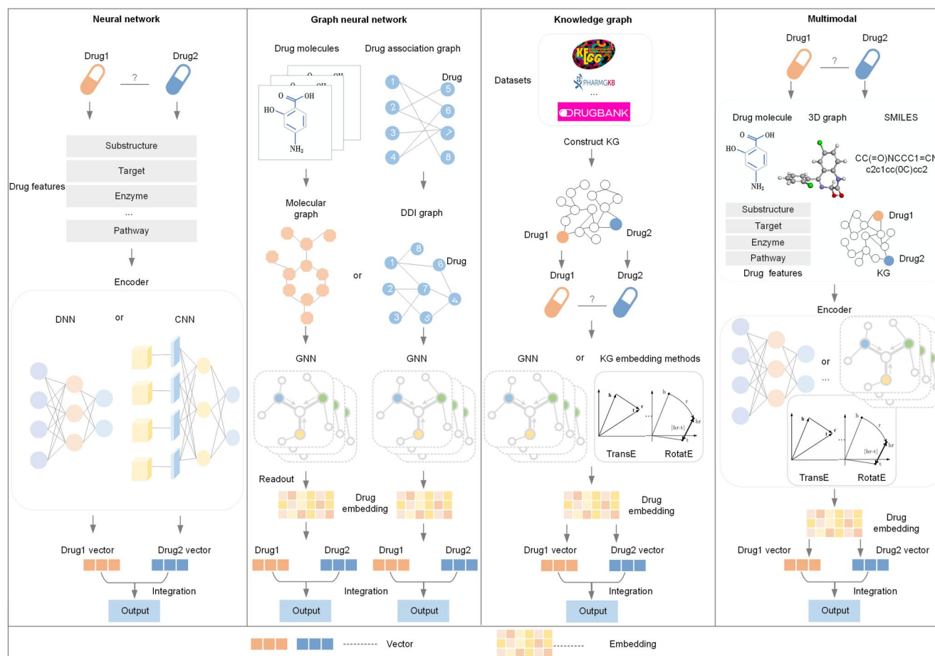
FIGURE 1 The overall workflow of four kinds of deep learning methods for DDIs prediction.
